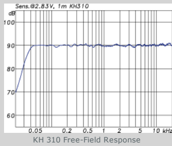
KH 310 Free-Field Response
