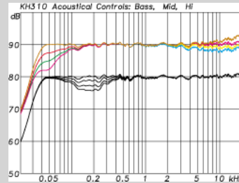
KH 310 Bass, Mid and High Acoustical Controls
