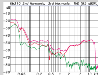
KH 310 Harmonic Distortion at 95 dB SPL (Purple: THD, Red: 2nd harmonic, Green: 3rd harmonic)
