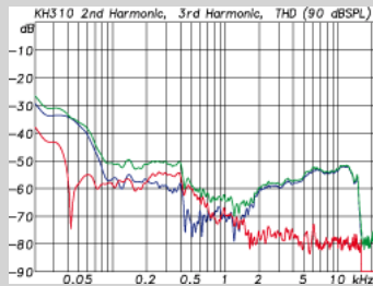
KH 310 Harmonic Distortion at 90 dB SPL (Green: THD, Blue: 2nd harmonic, Red: 3rd harmonic)
