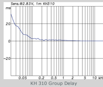
KH 310 Group Delay
