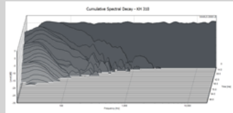
KH 310 Cumulative Spectral Decay
