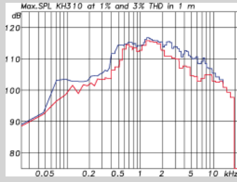
KH 310 Maximum SPL at 1m (Red: 3% THD, Blue: 1% THD)
