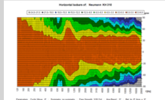
KH 310 Horizontal Directivity Plot
