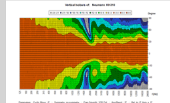
KH 310 Vertical Directivity Plot
