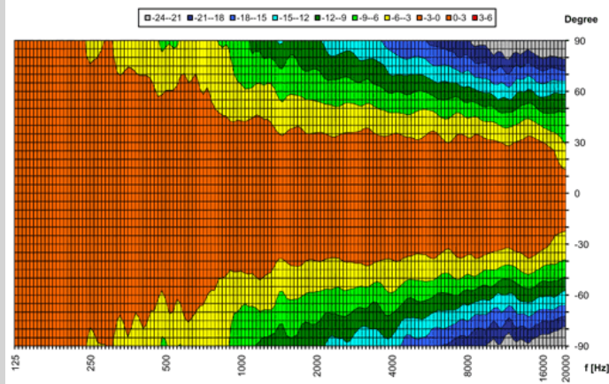
KH 120 Horizontal Directivity Plot
