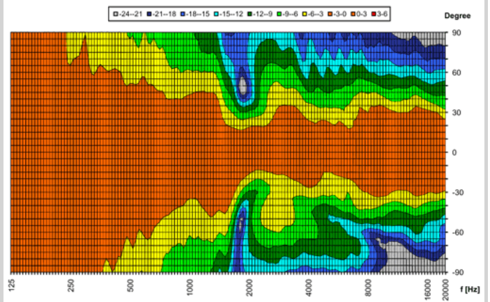
KH 120 Vertical Directivity Plot
